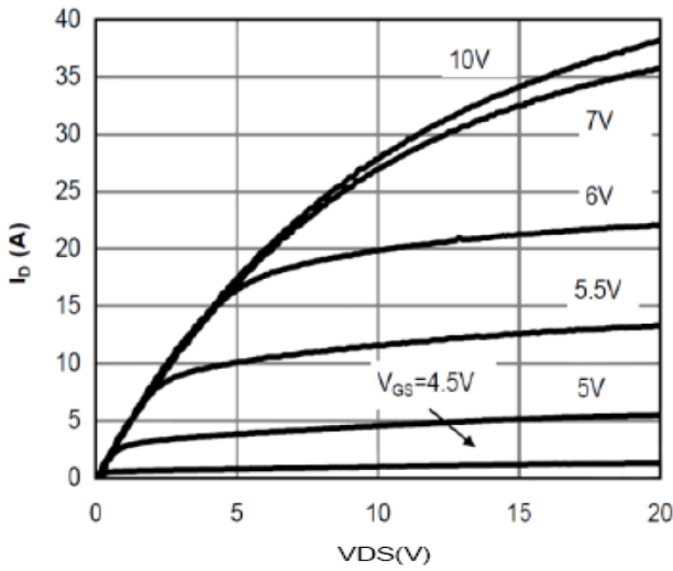
Output Characteristic
