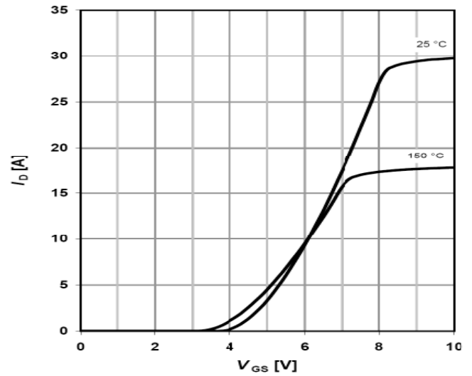
Transfer Characteristic
