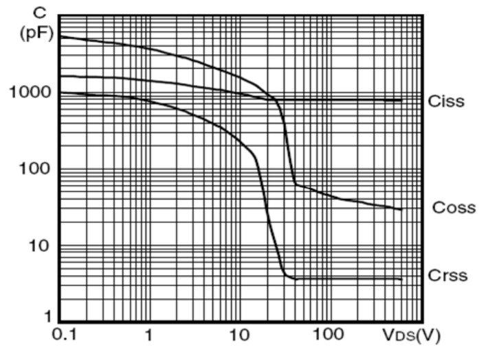
Capacitance
