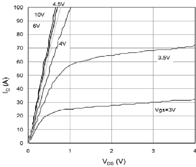
Output Characteristics
