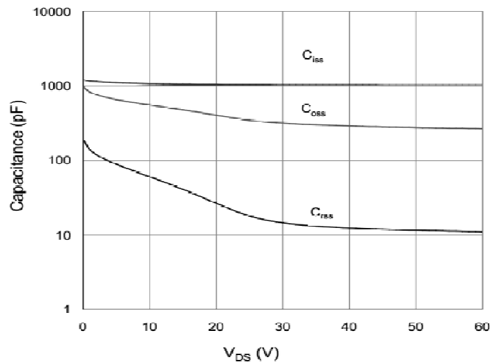
Capacitance
