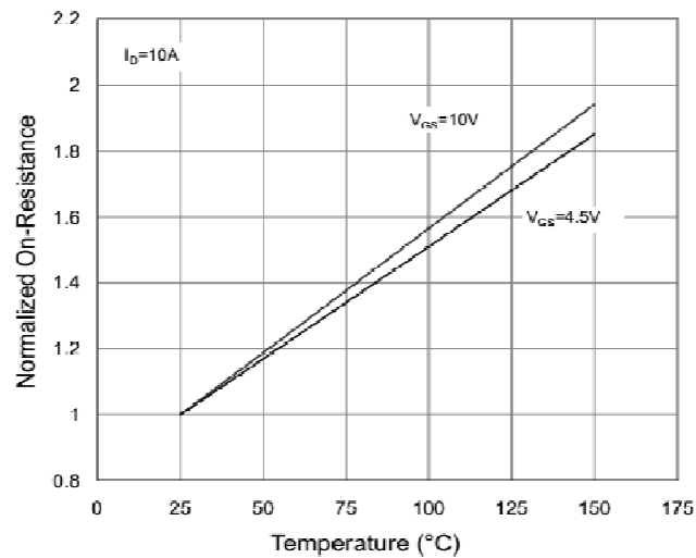
Rdson-JunctionTemperature
