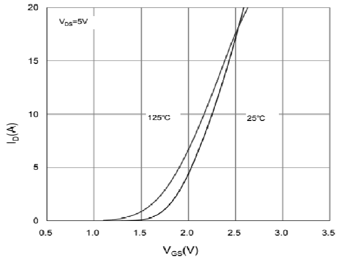
Transfer Characteristics
