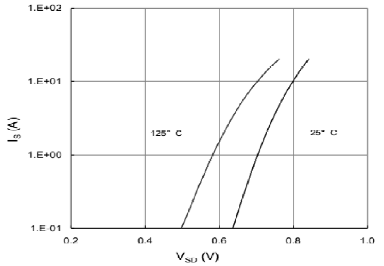
Source-Drain Diode Forward Voltage
