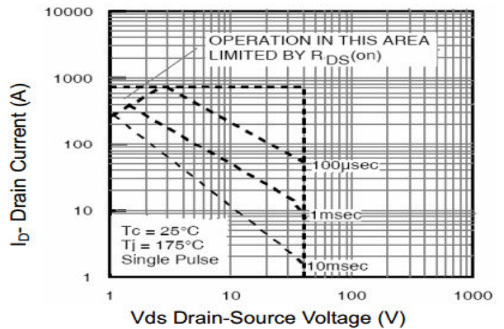
Safe Operation Area
