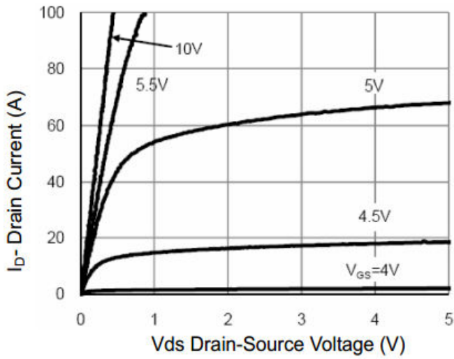
Output Characteristic
