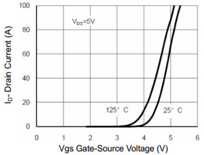
Transfer Characteristic
